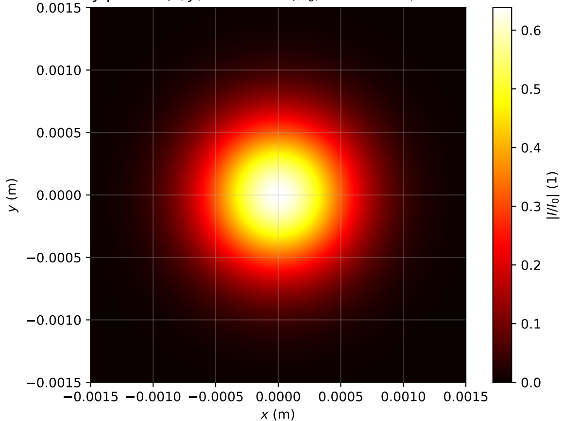
Intensity profile I(x, y, z = 1.831m)/I_0 , \text{Pin}=0.2\text{Pcr} , artificial time
